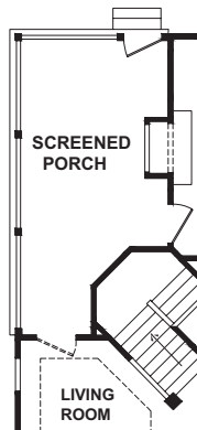
SCREENED PORCH OPTION 1 AND 2-SIDED FIREPLACE OPT.
