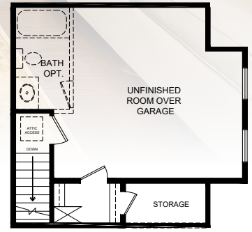
SECOND FLOOR PLAN ROOM OVER GARAGE
