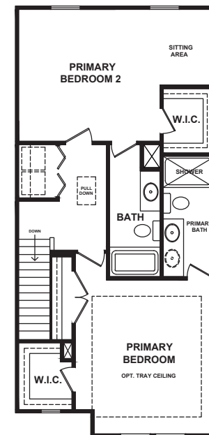
Second Floor With Optional Dual Primary Suites
